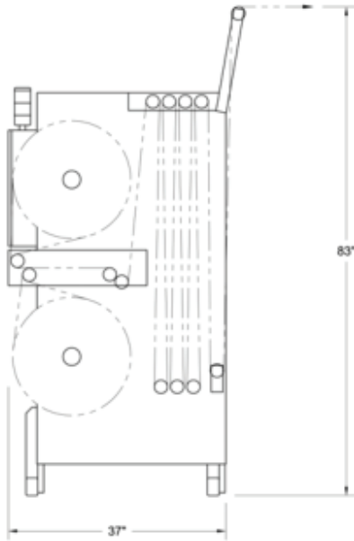
MODEL PS1220-03 DIMENSIONS SUBJECT TO CHANGE WITHOUT NOTICE
