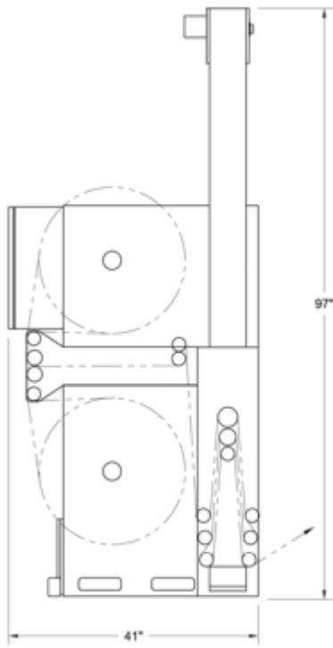
MODEL PA1624-05
